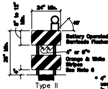
PORTABLE FLASHER SUPPORT BARRIOLE
