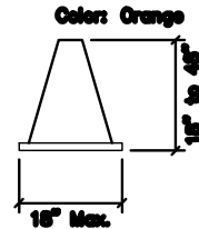
CONE DELINEATOR
