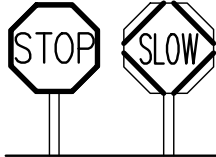
(C18) (C18) 12 White on Red and Black on Orange on Black 24" x 24"-S Series C Letters 15" x 15"-S Series C Letters Non-ReflectORIZED
